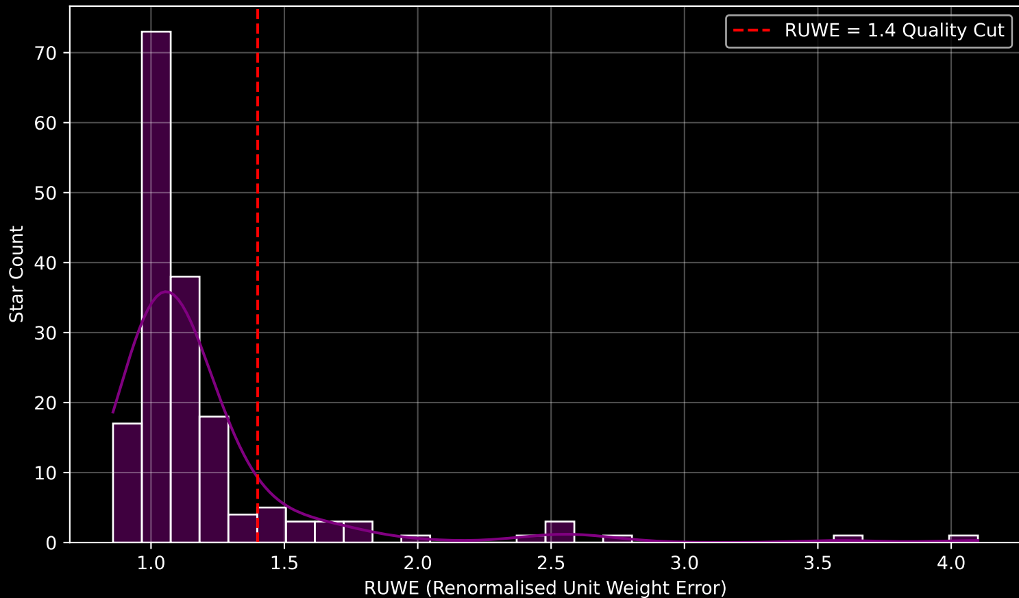
GAPOGEE DR17 Field [170-23-O] RUWE Distribution (n= 172)
