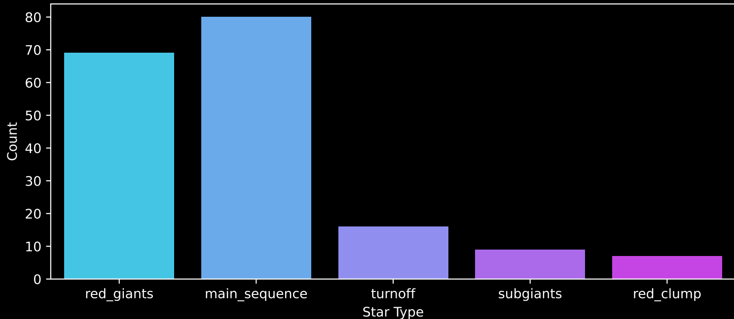
APOGEE DR17 Field: [170-23-O] Count plot of Star Type
