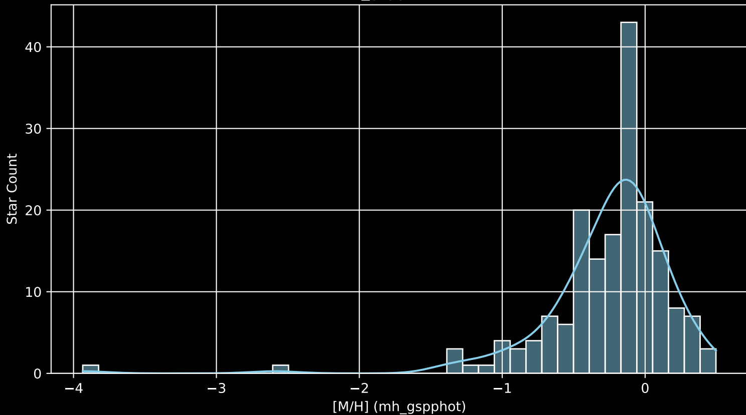
APOGEE DR17 Field: [170-23-O [M/H] (mh_gspphot) (n= 179)
