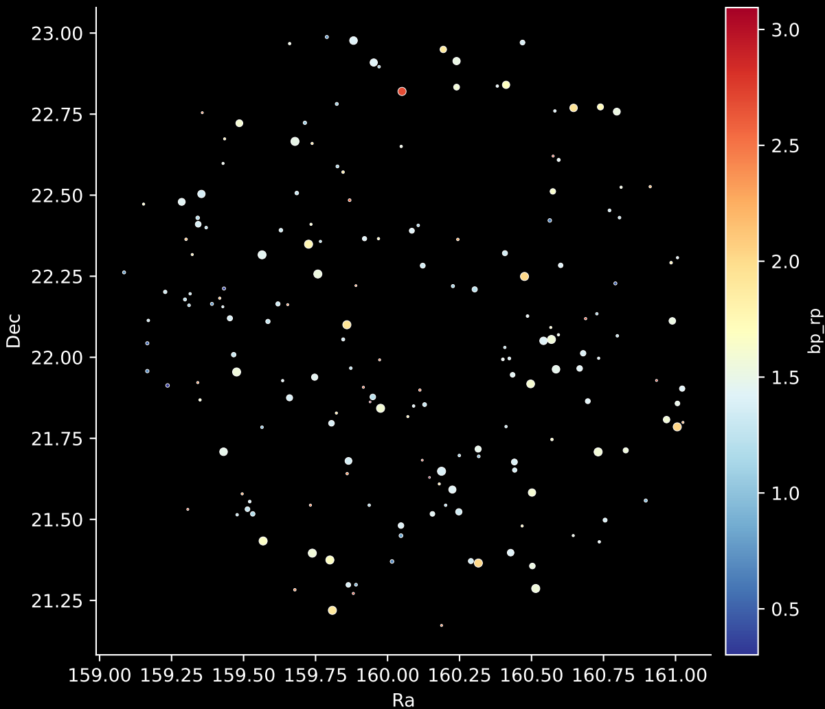
APOGEE DR17 Field: [170-23-O] Stars: 181
