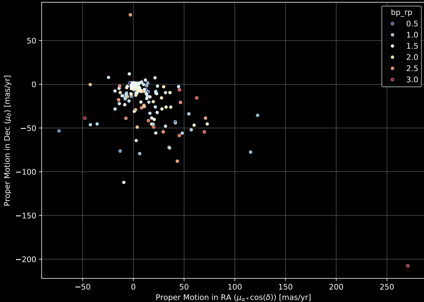
APOGEE DR17 Field: [170-23-O] Proper Motion Diagram (n= 181)
