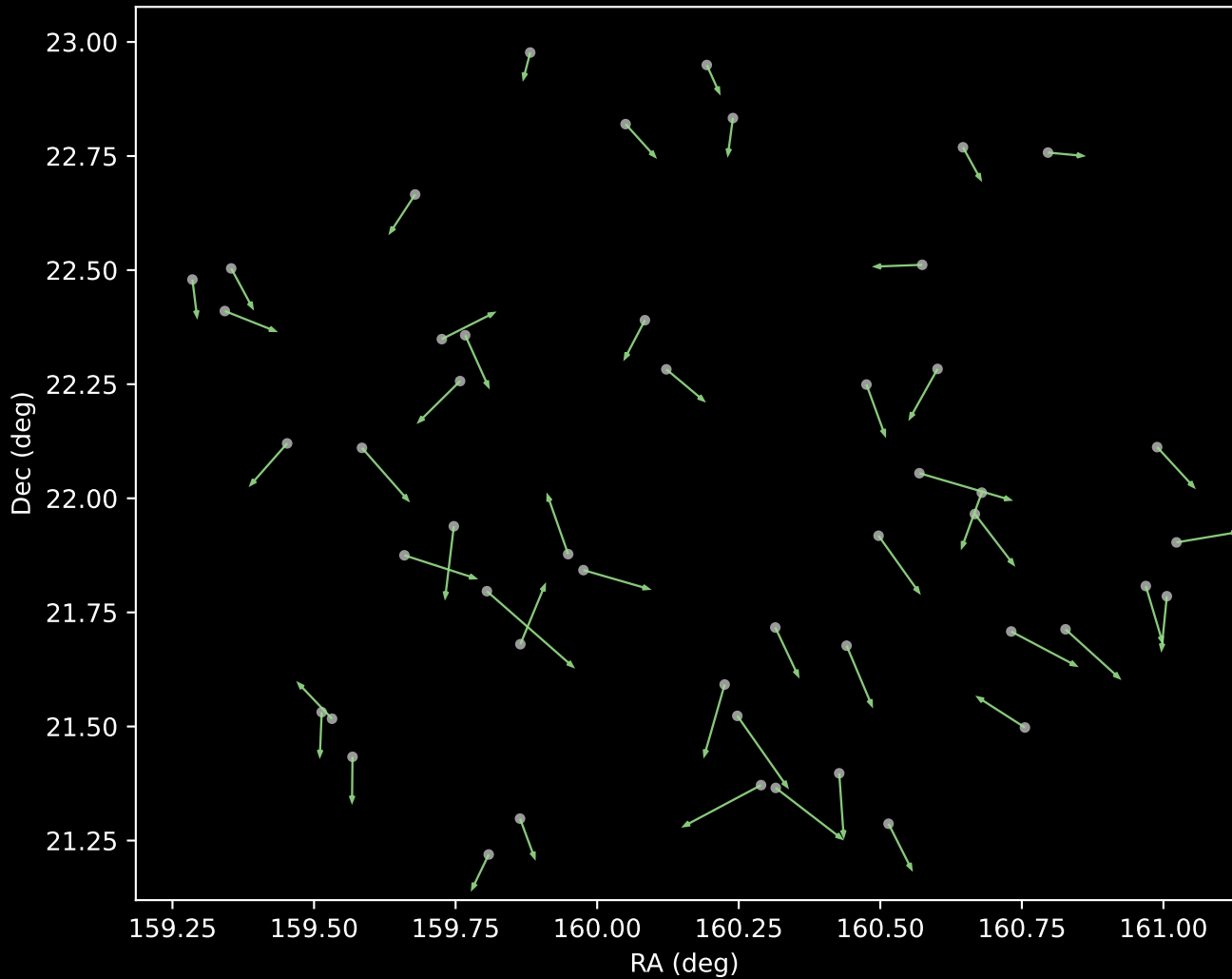
APOGEE DR17 Cluster 5 Proper Motion Vectors (n=50)
