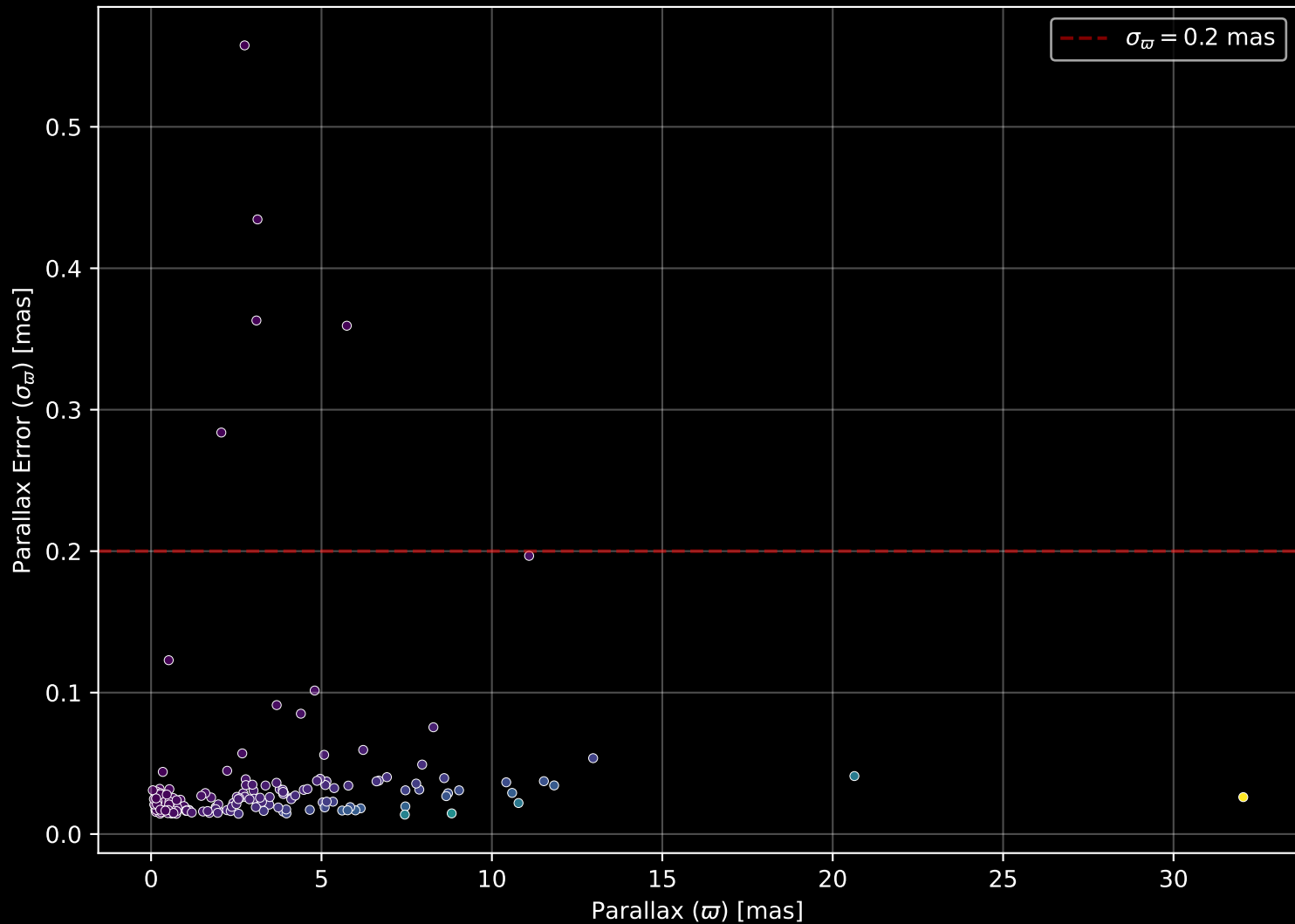
APOGEE DR17 Field: [170-23-O] Parallax Quality (n= 181)
